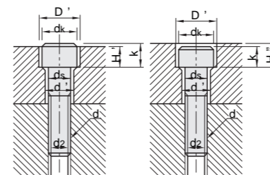
Reference Dimensions of counterboring and bolt hole for the socket head cap screws
